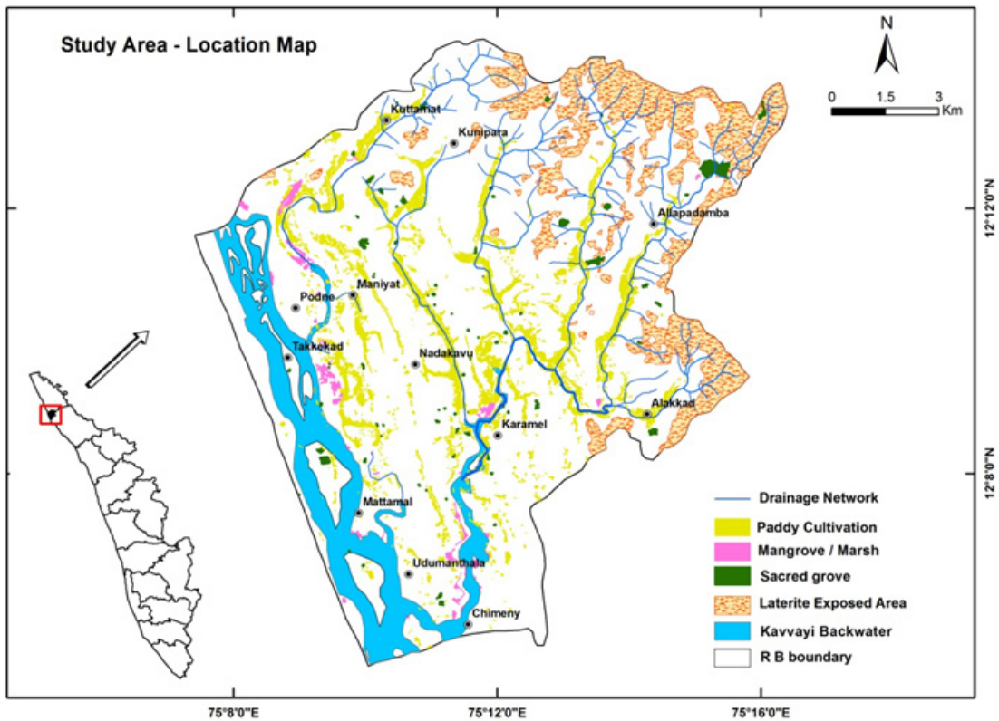
Fig. i: Location map of Kavvayi river basin showing critical land cover
